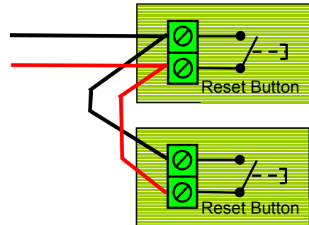
Circuit Diagram of two switches
